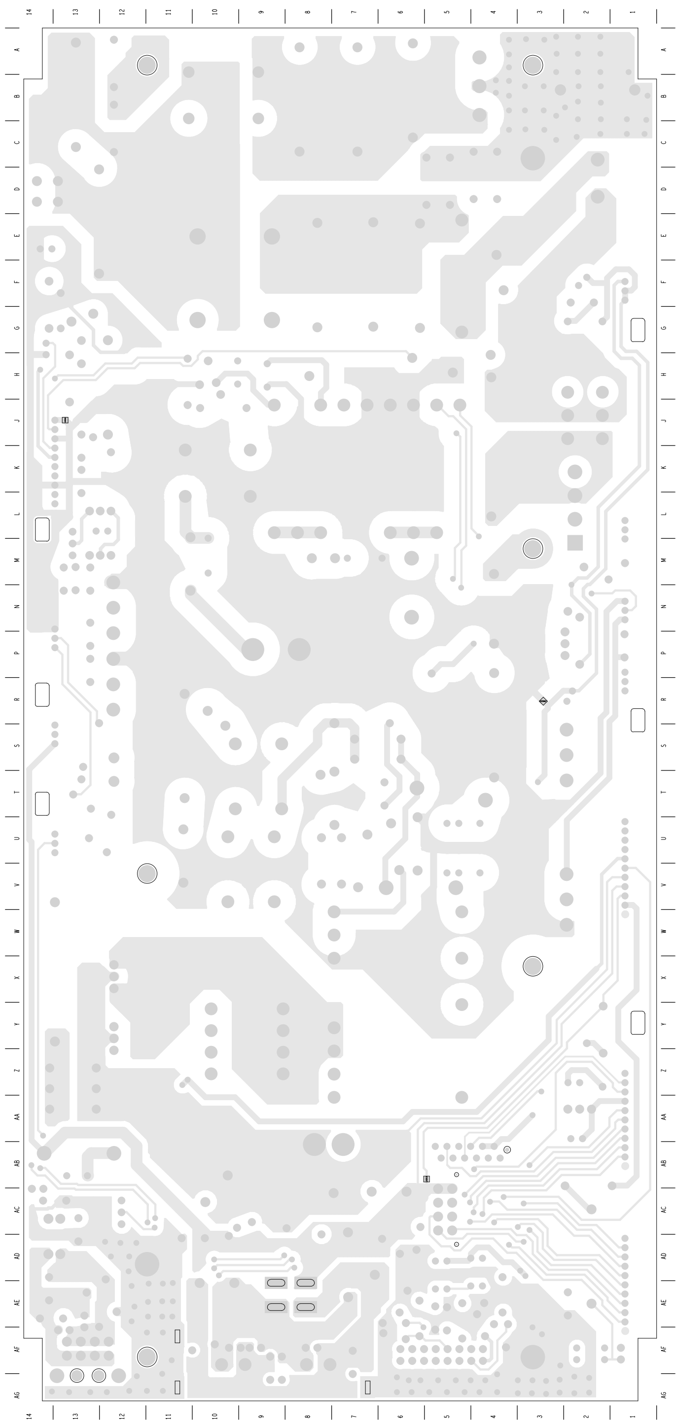
TAIT ELECTRONICS P/N: 220-02017-17 D: 14Jun05 MCL: NLS TB8000 AC-DC CONVERTER PCB LAYOUT-SECONDARY-SIDE
